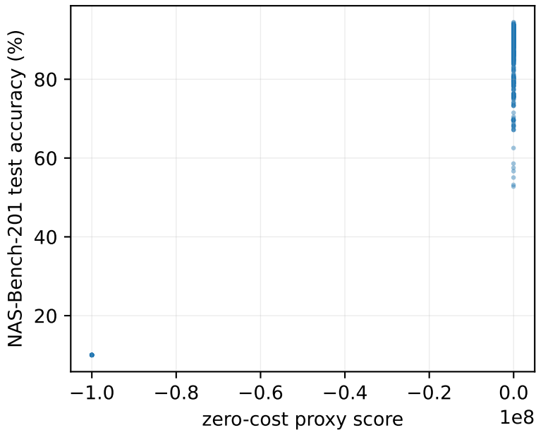
comparative-1-jacobcov-cifar10
