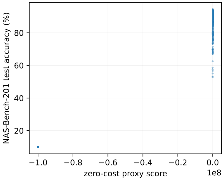
comparative-4-jacobcov-cifar10rep
