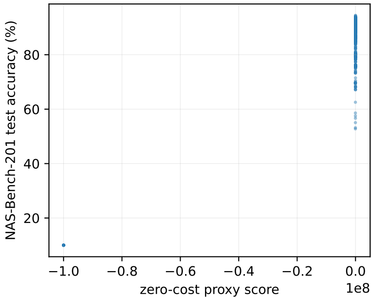
comparative-2-jacobcov-pixshuf
