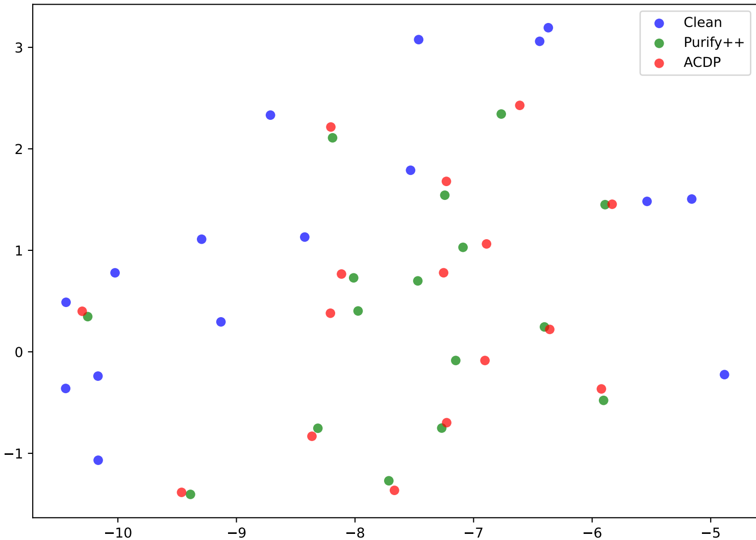
t-SNE of Feature Space for Different Image Types
