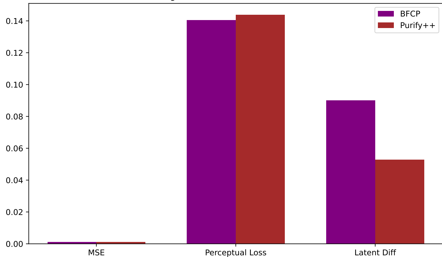
Average Semantic Preservation Metrics
