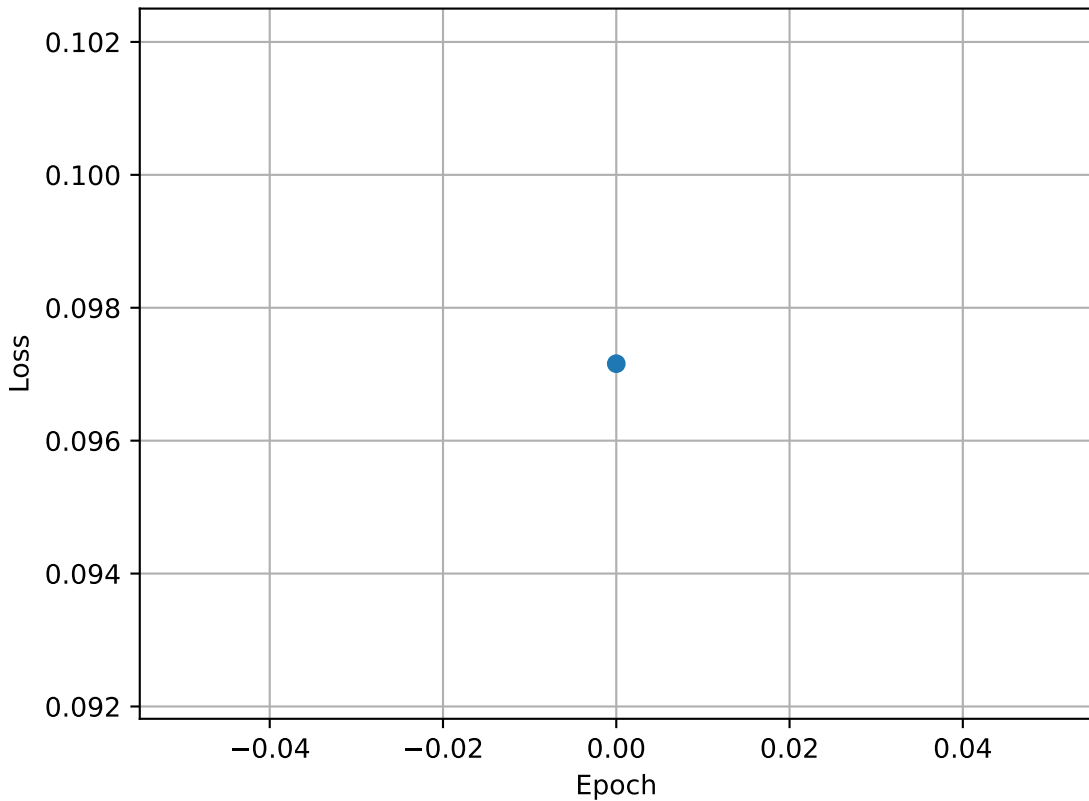
TRExFiT + Consistency
