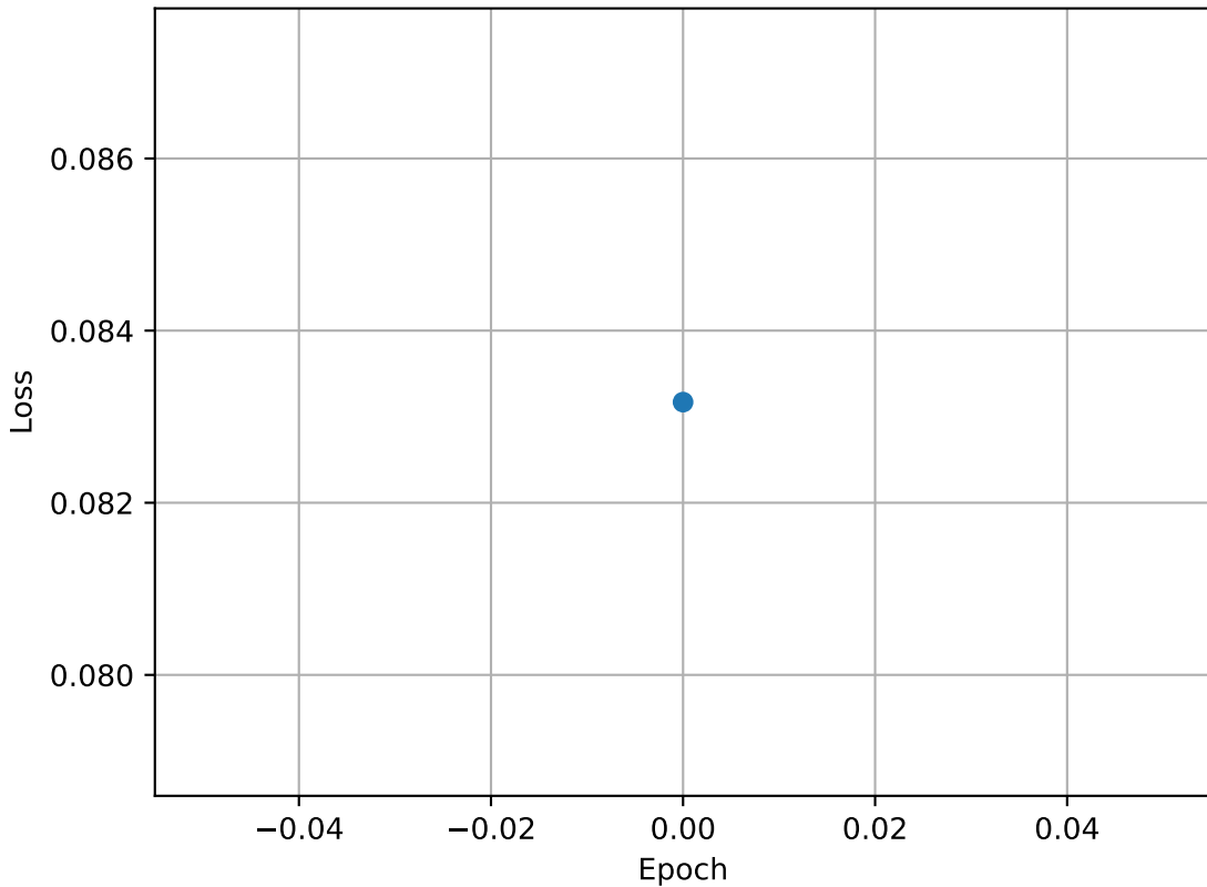
TRExFit Standard
