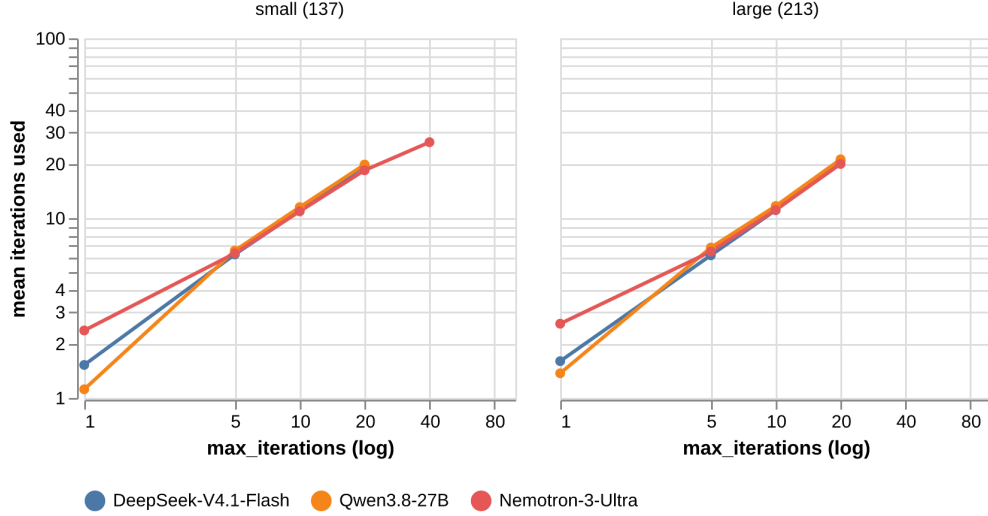
Mean iterations used vs iteration budget (runs finished by v1)
