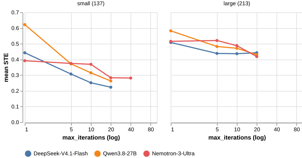
Mean STE vs iteration budget (lower is better; runs finished by v1)
