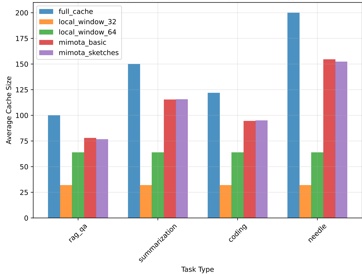
Memory Usage by Cache Management Strategy
