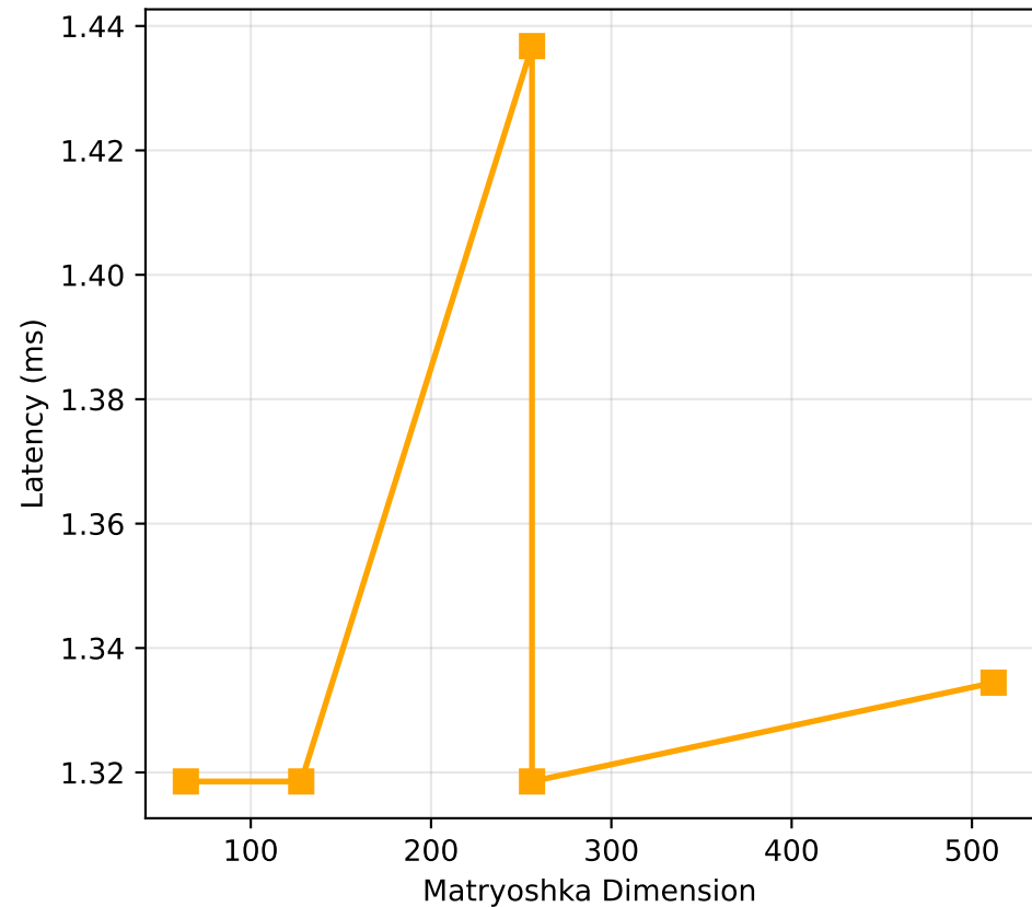
Latency vs Retrieval Dimension
