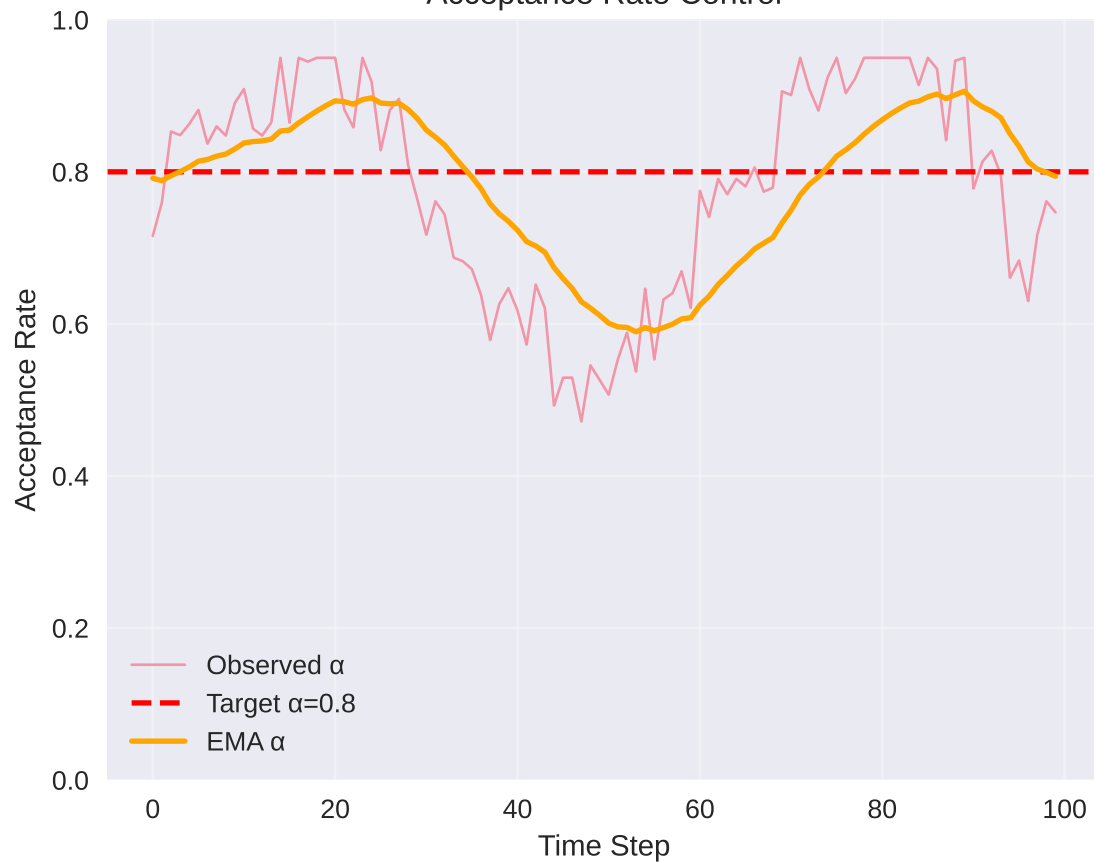
Adaptive Draft Configuration
