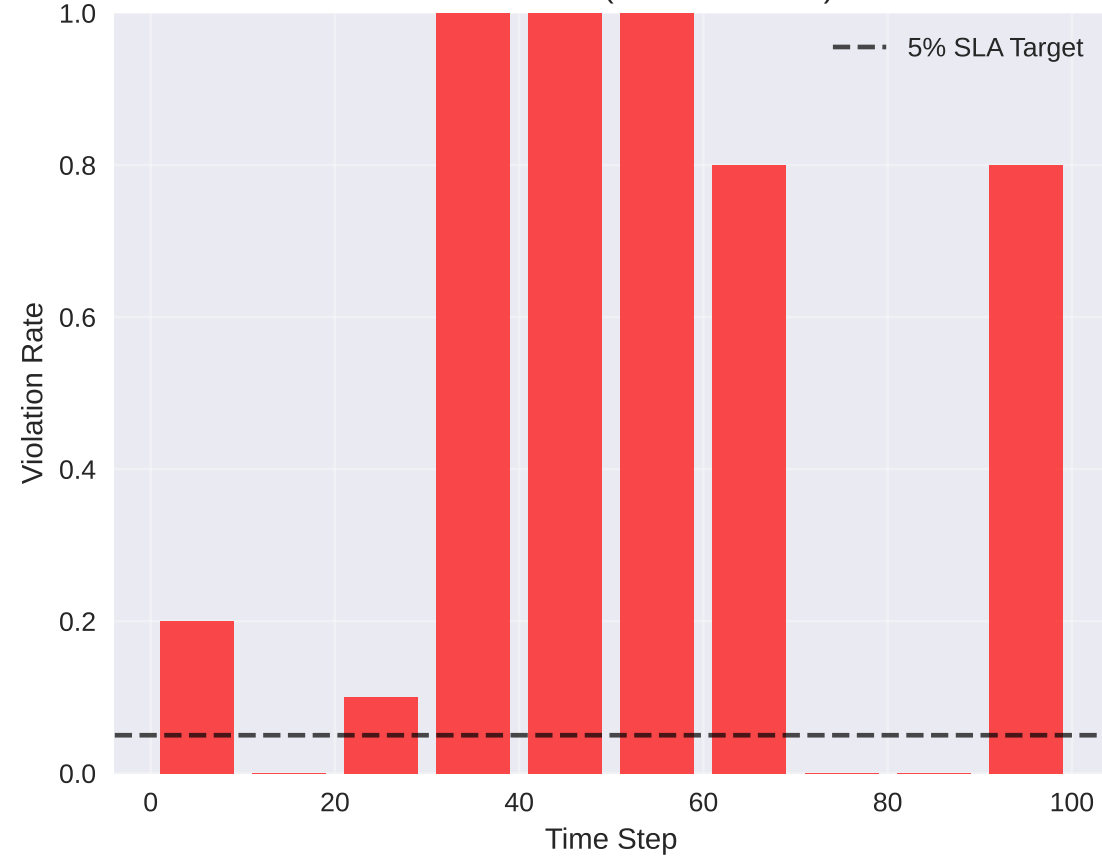
SLA Violations (Overall: 49.0%)
