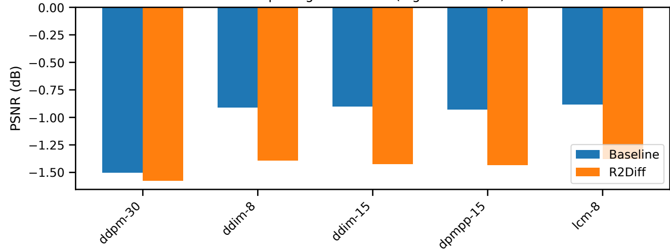
Sampler-agnostic PSNR (higher is better)
