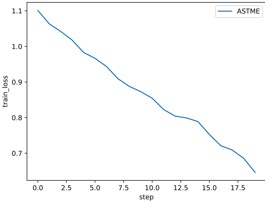
Training Loss - ASTME
