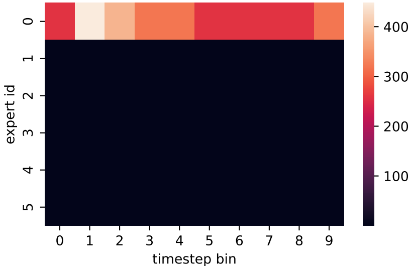
Expert vs Timestep counts (full ASTME)
