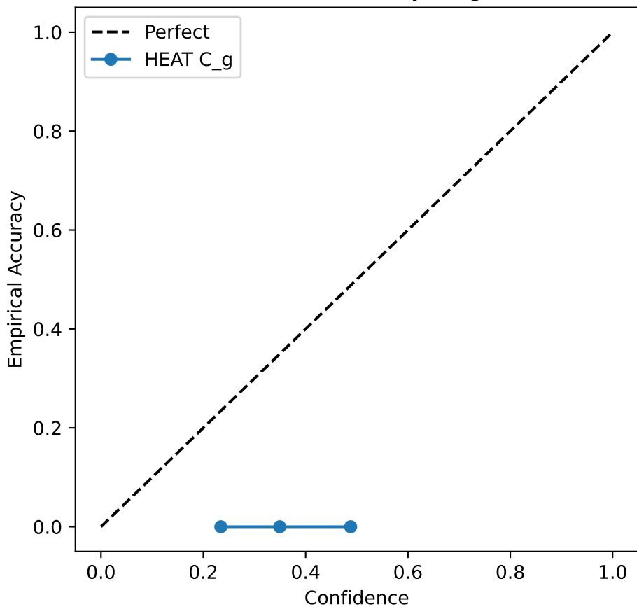
Calibration Reliability Diagram
