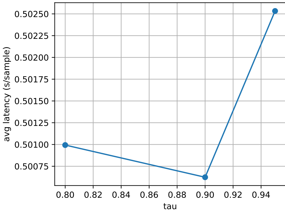
Summarization Latency vs tau (mini)
