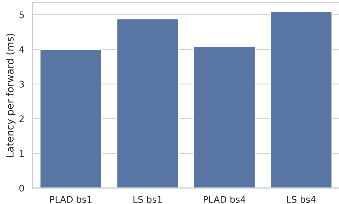
Inference latency (uniform)
