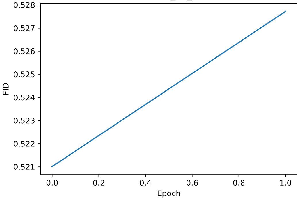
FID - fft_dit_xs
