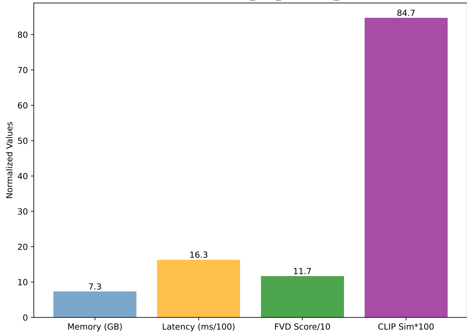
Video Performance: Jetson_Orin_8GB - limit_adaptive
