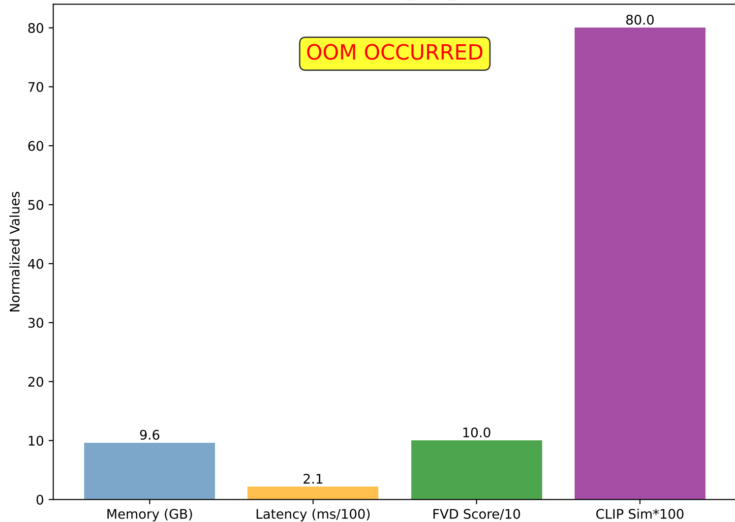
Video Performance: Jetson_Orin_8GB - deepcache
