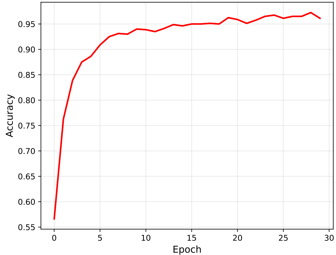
Training Accuracy
