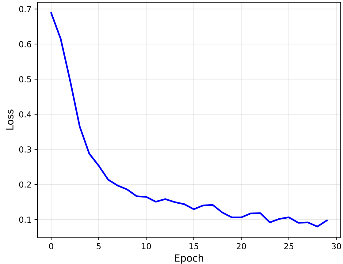
Training Loss
