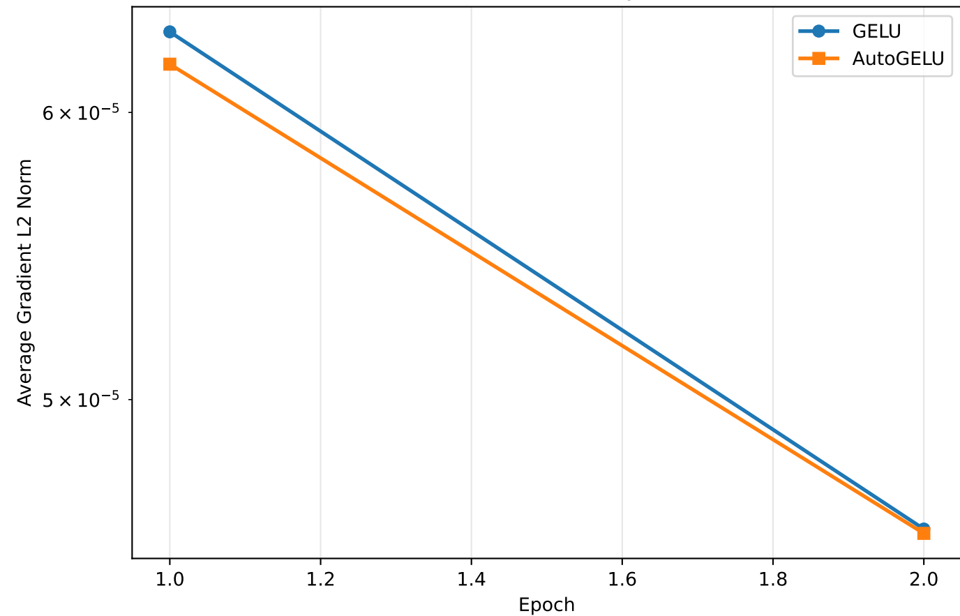
Average Gradient Norm Across All Layers
