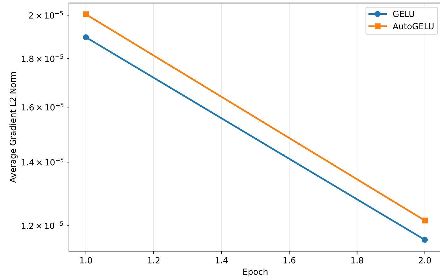
Gradient Flow in Layer 10
