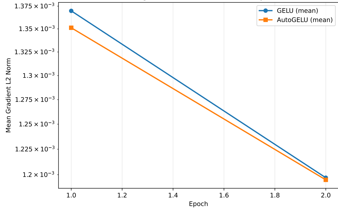
Average Gradient Norm Across All Layers
