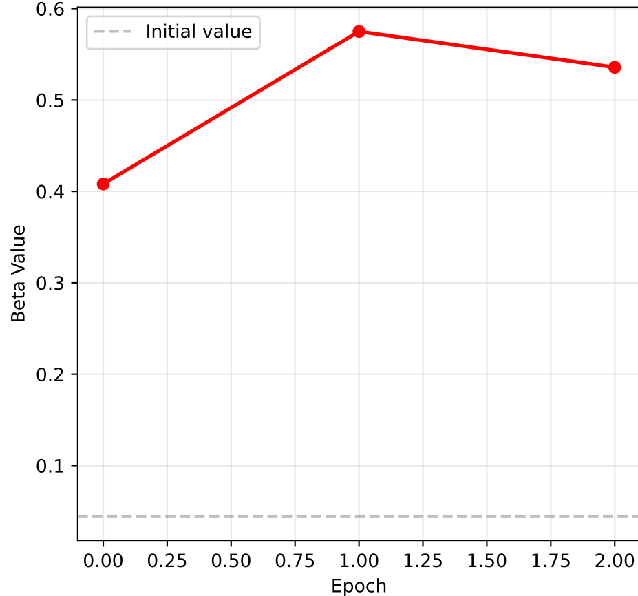
Evolution of AutoGELU Beta
