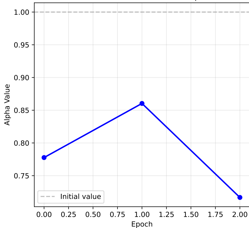
Evolution of AutoGELU Alpha
