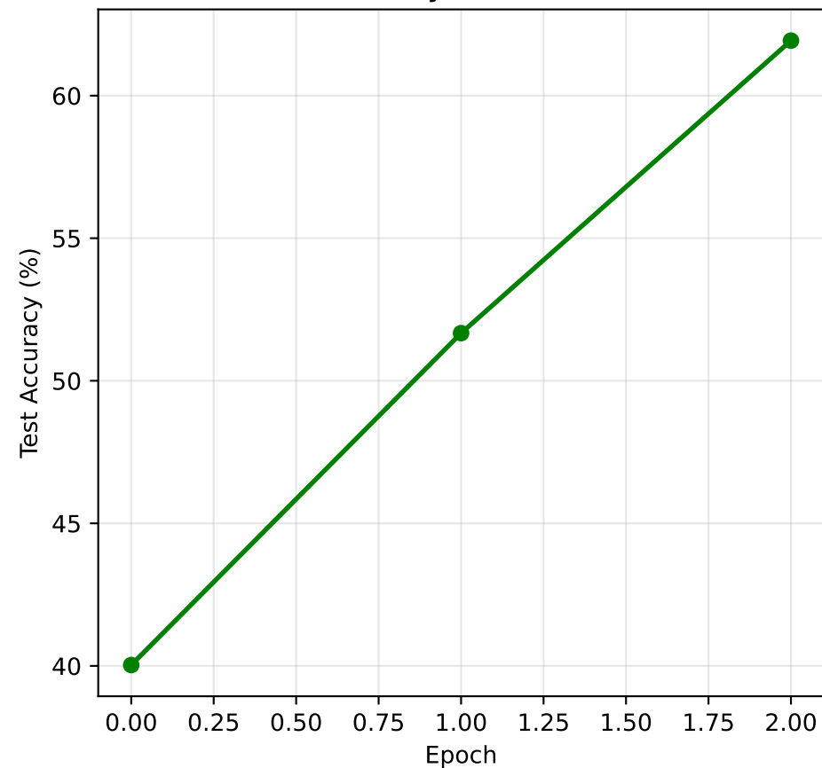
Test Accuracy with AutoGELU
