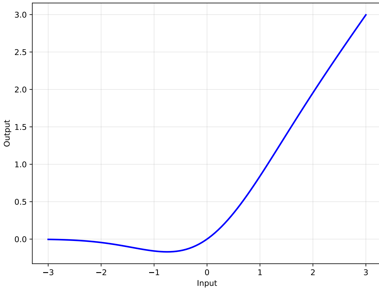
AutoGELU Activation Function
