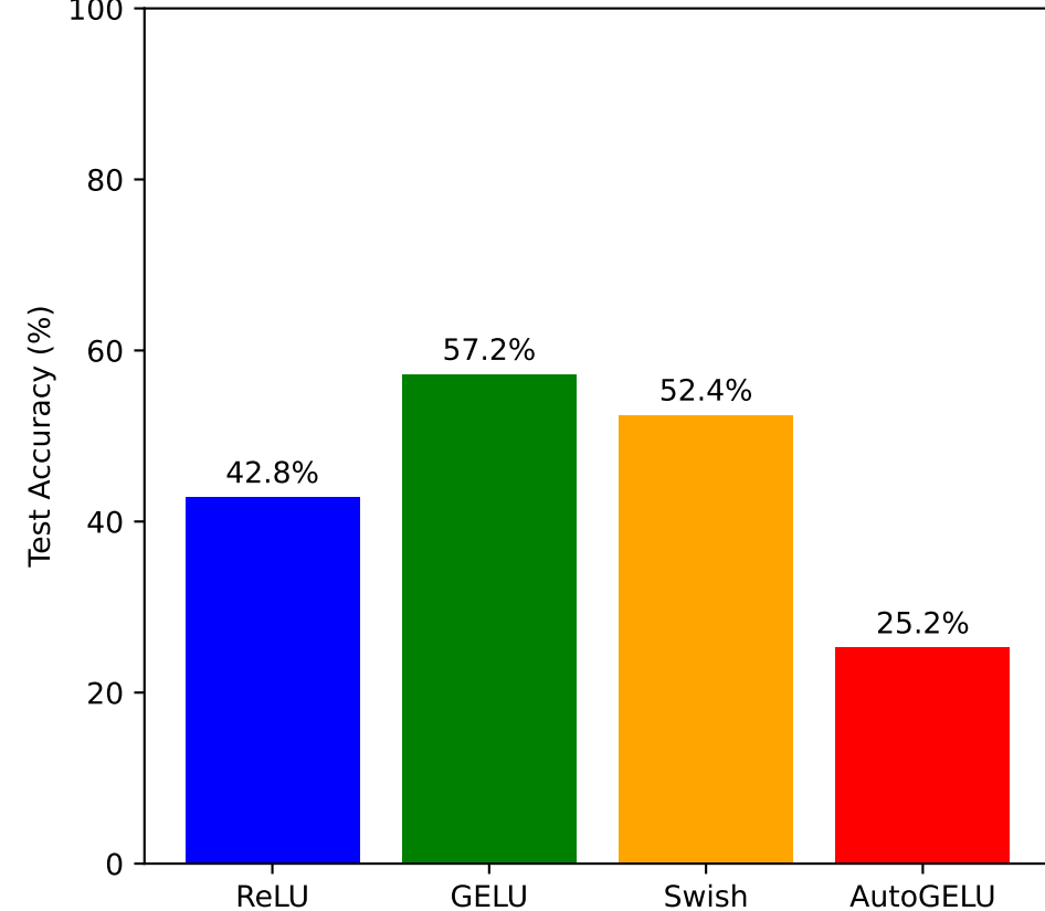
Final Test Accuracy
