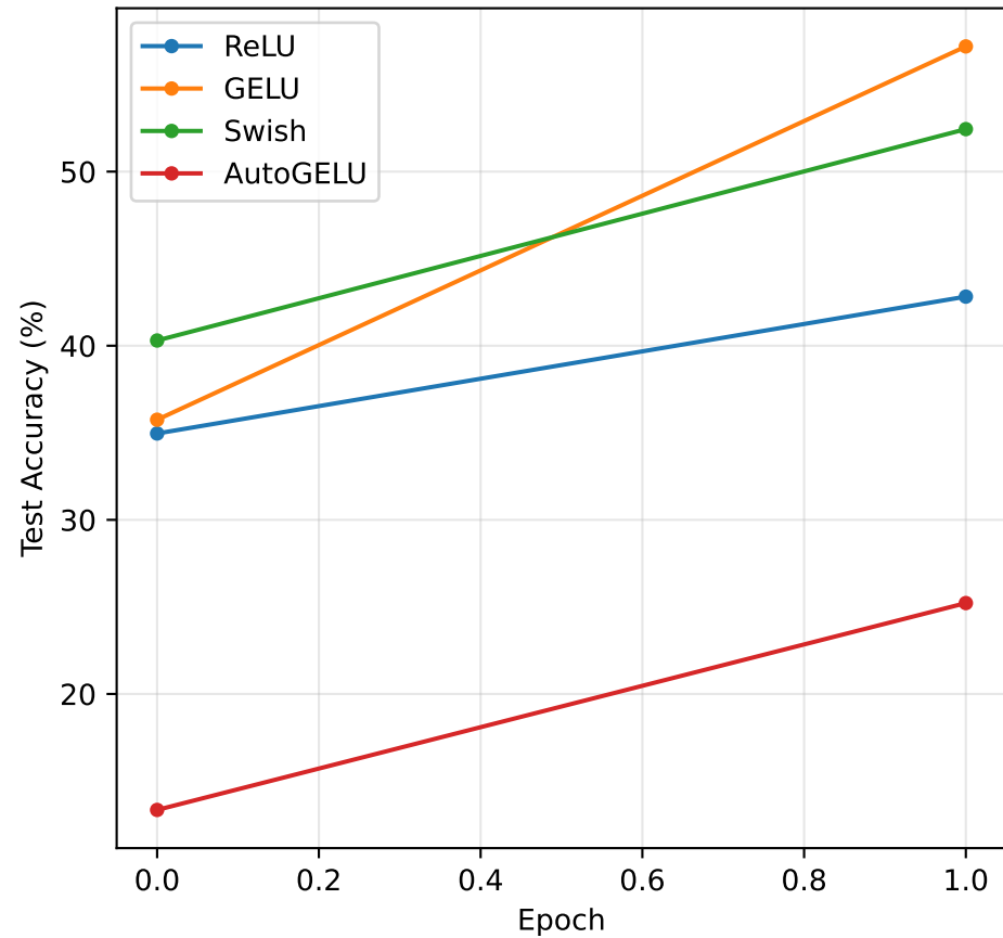
Test Accuracy Comparison
