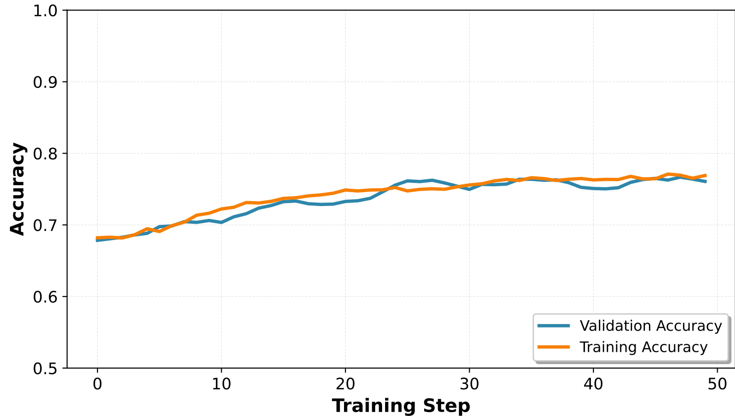
Comparative 1 Clip: Rn50 on Caltech-101
