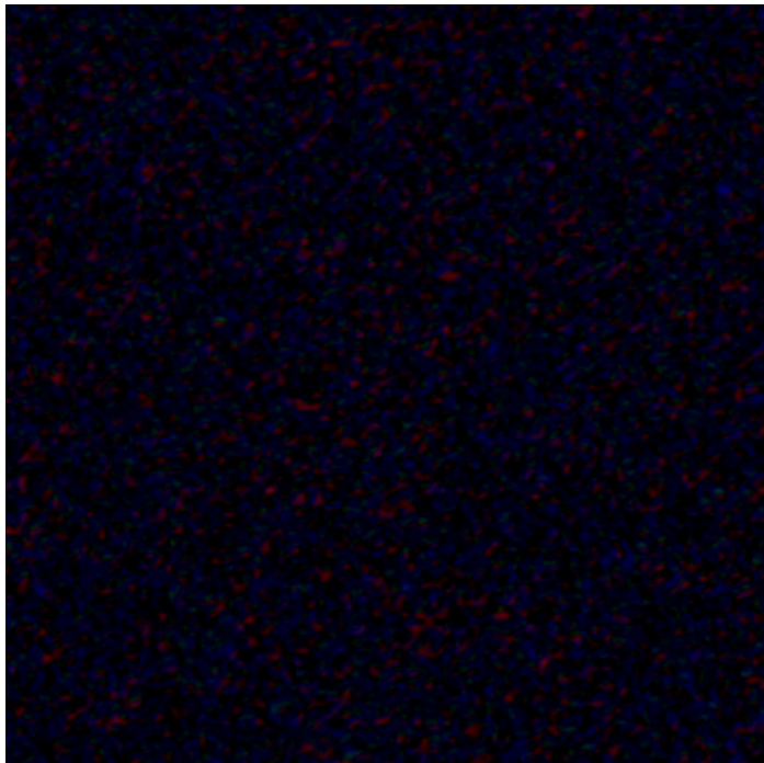
FiT 512x512
