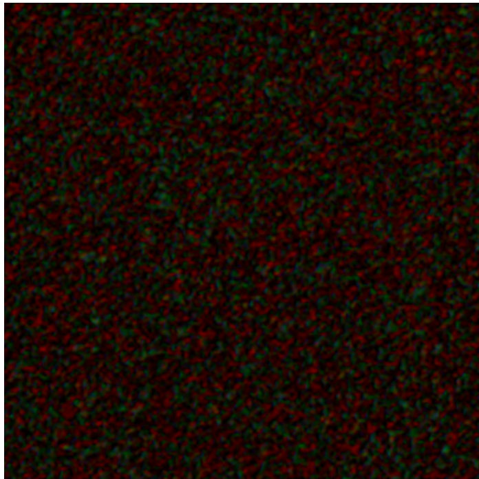
FaFT 512x512
