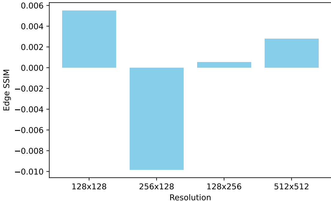
Edge SSIM between FiT and FaFT across Resolutions
