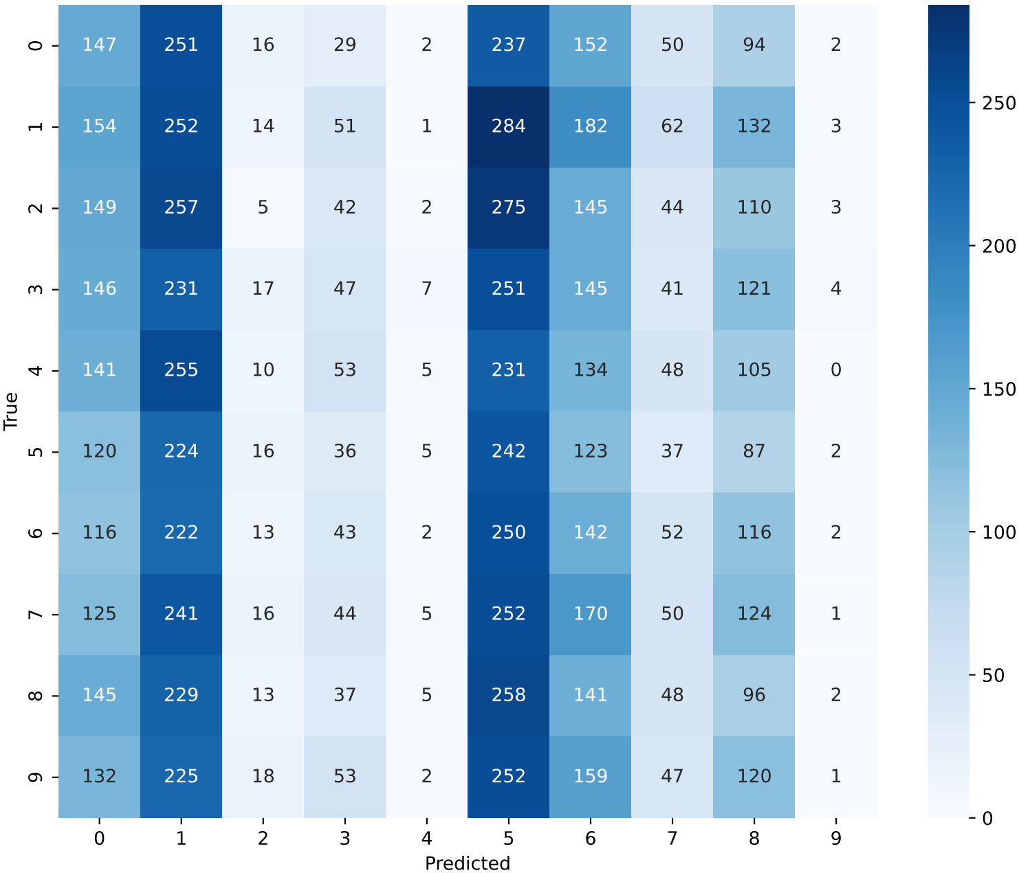
Confusion Matrix (ACM)
