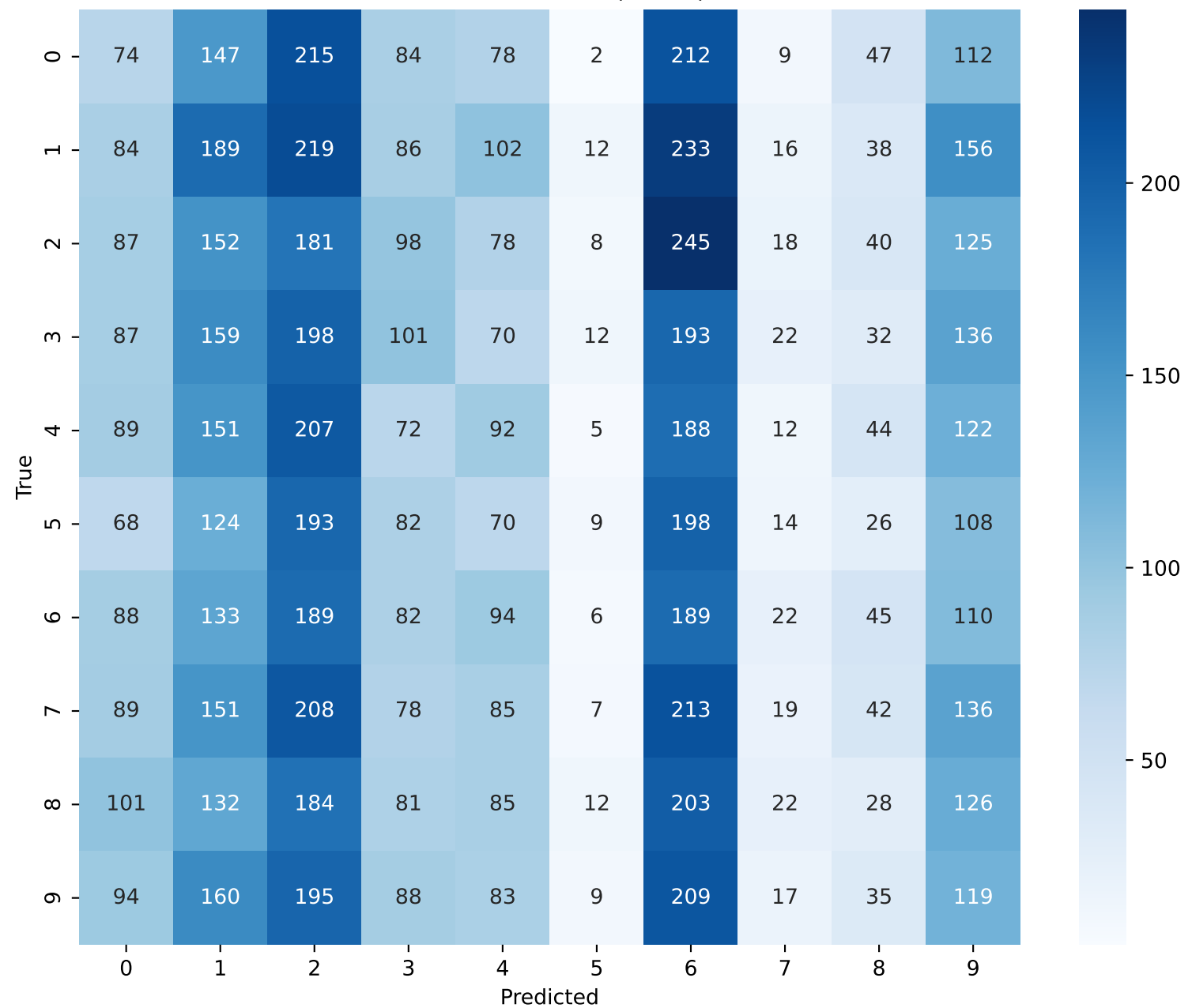
Confusion Matrix (Adam)
