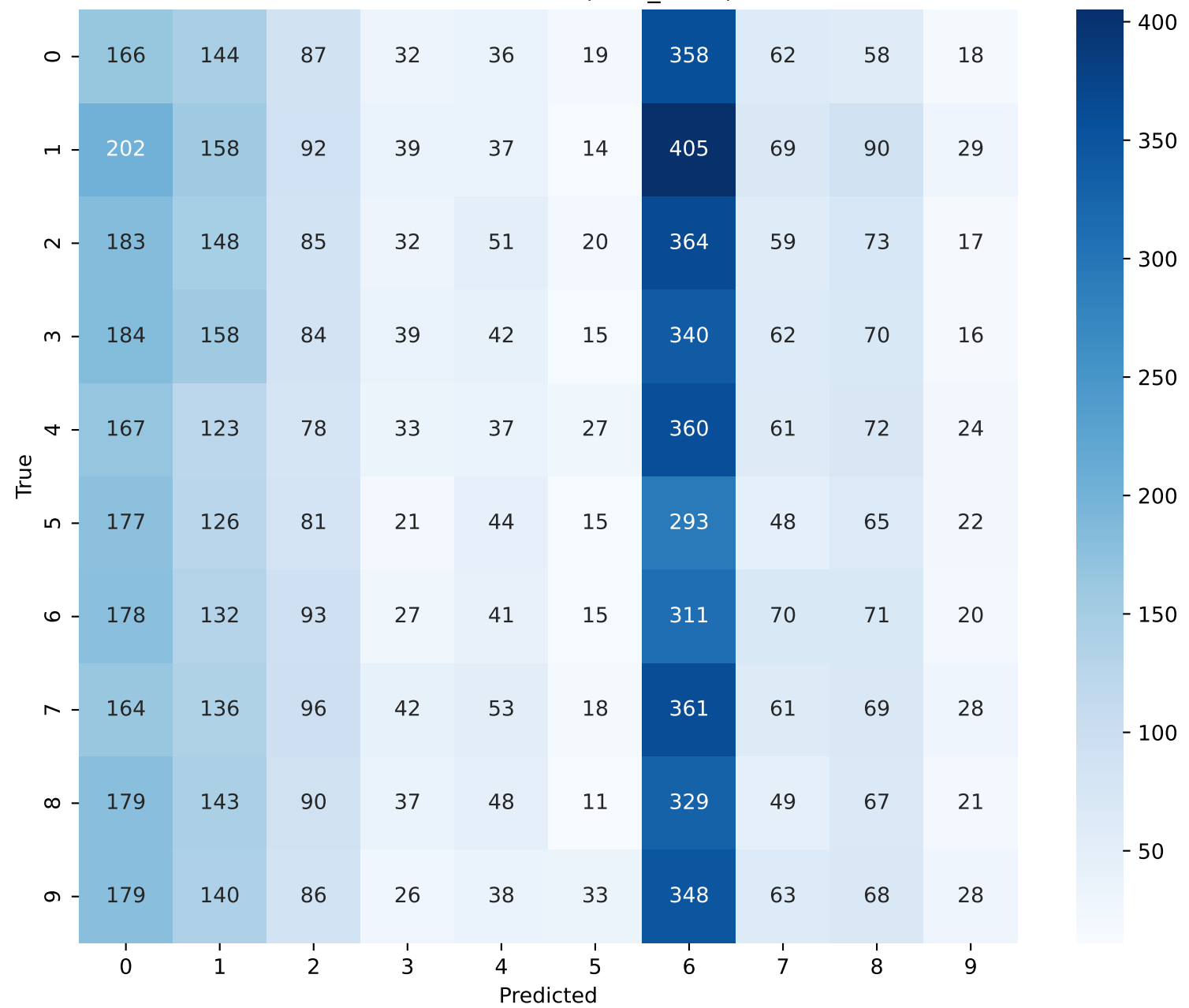
Confusion Matrix (SGD_mom)
