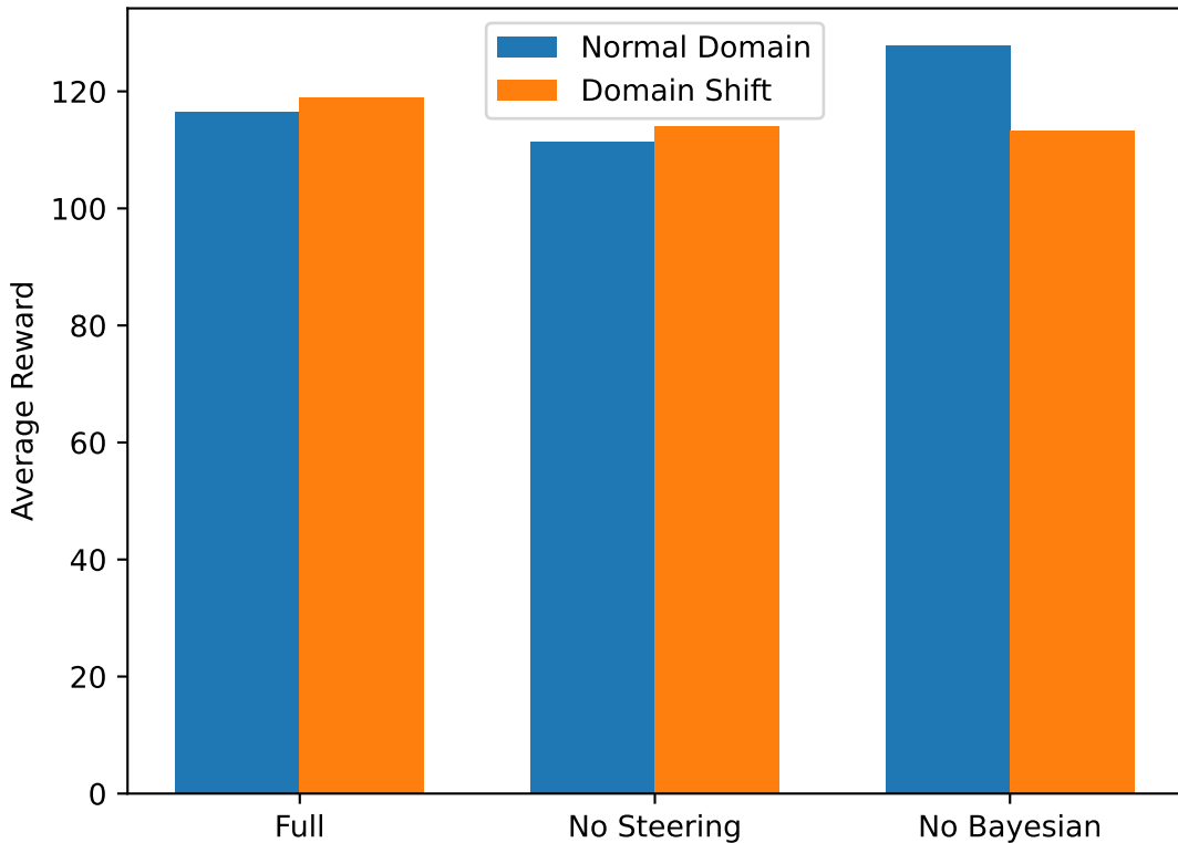
Ablation Study: Domain Performance
