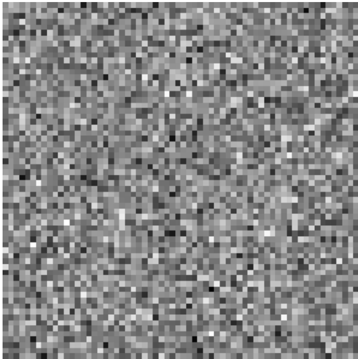
ILWGAN Interp
