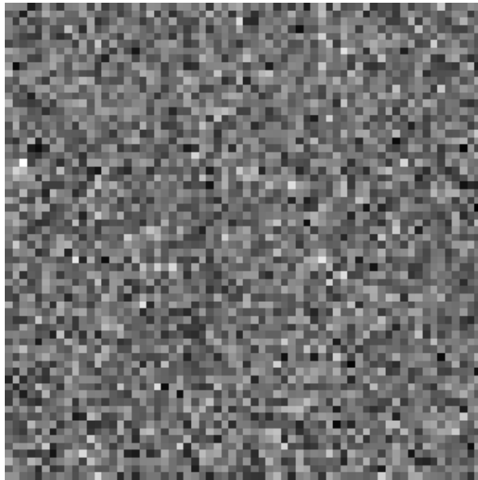
LWGAN Interp
