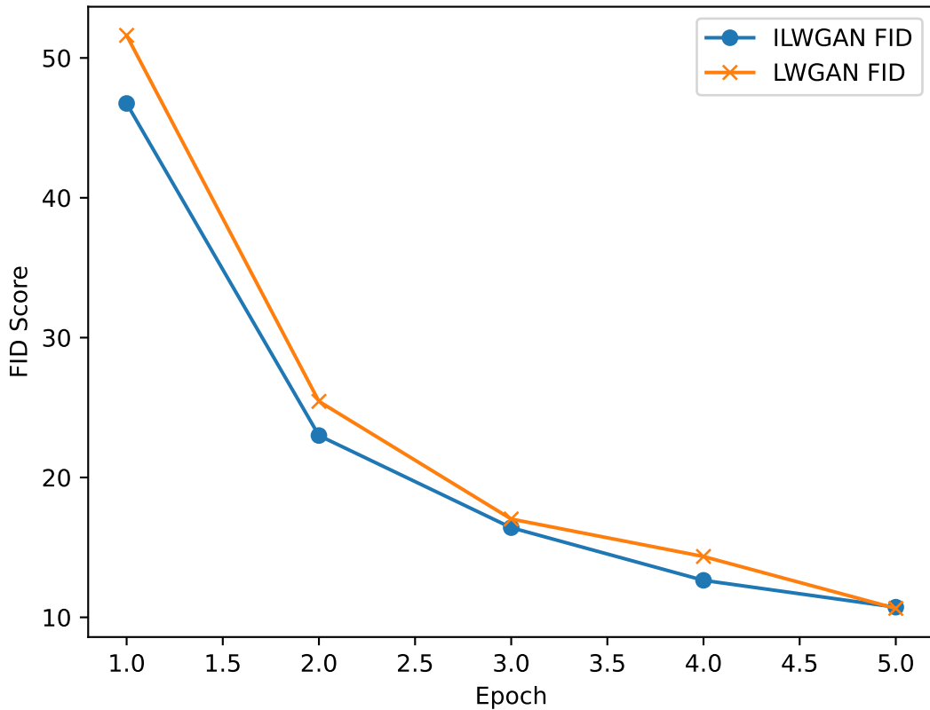
FID Scores Over Training
