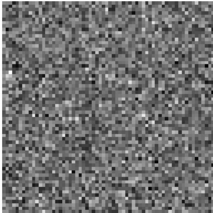
LWGAN Interp
