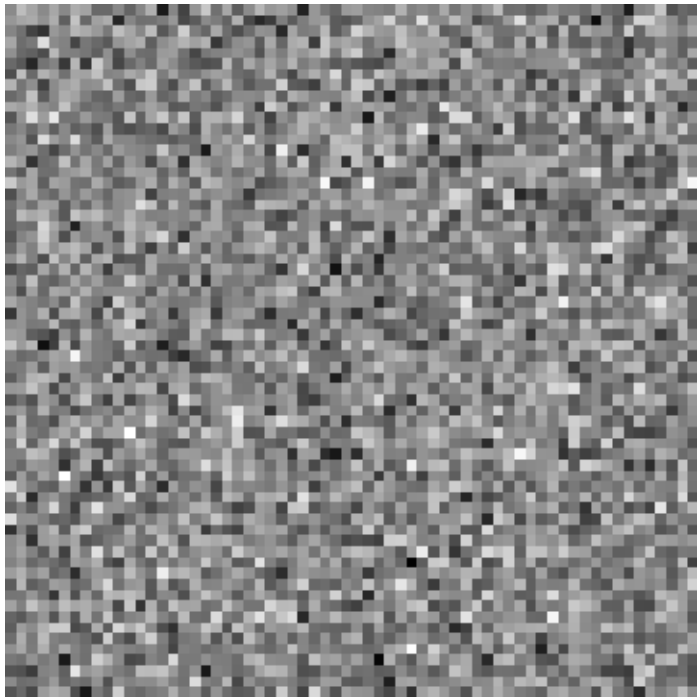
ILWGAN Interp
