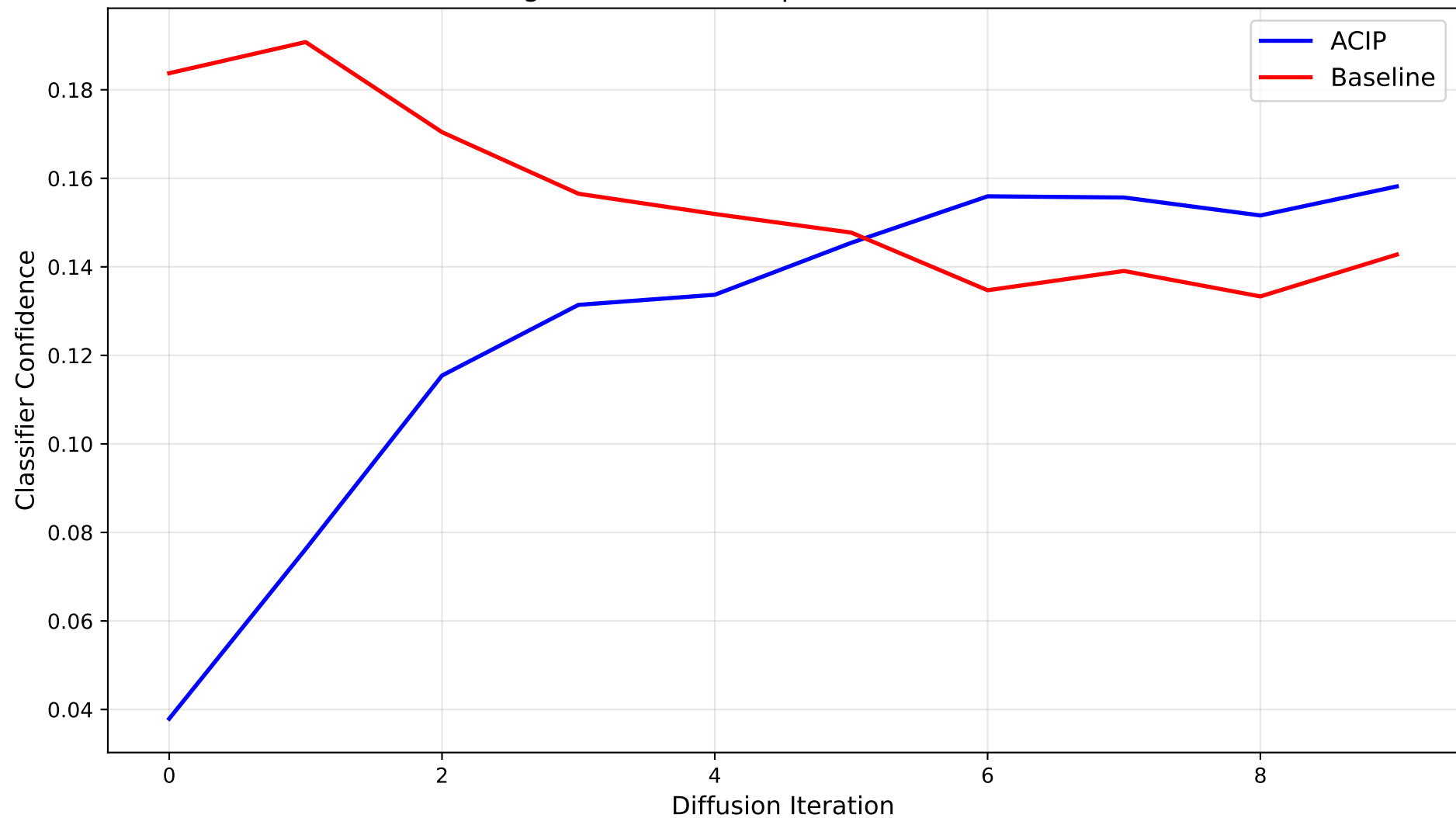
Convergence Curve Comparison: ACIP vs Baseline
