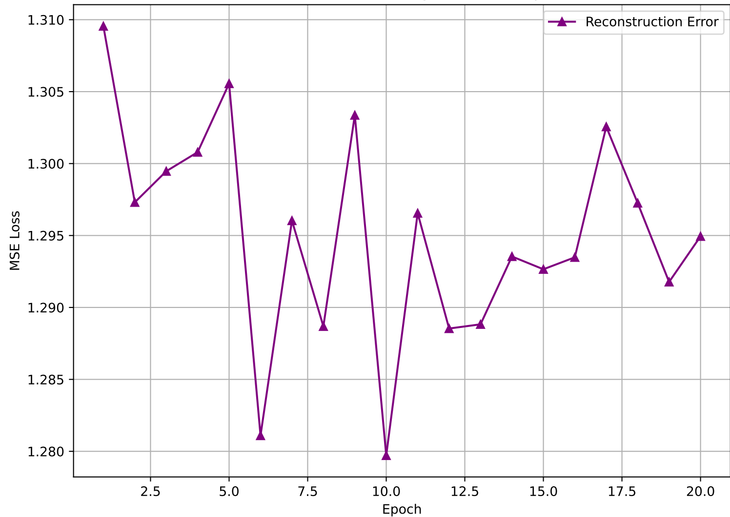
Reconstruction (Denoising) Error over Epochs
