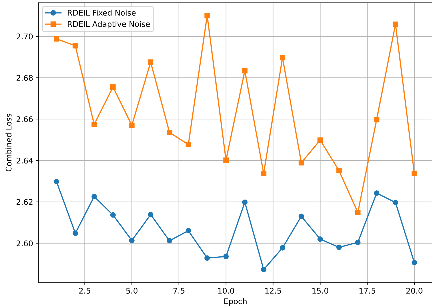
Training Loss Curves (Fixed vs Adaptive Noise)
