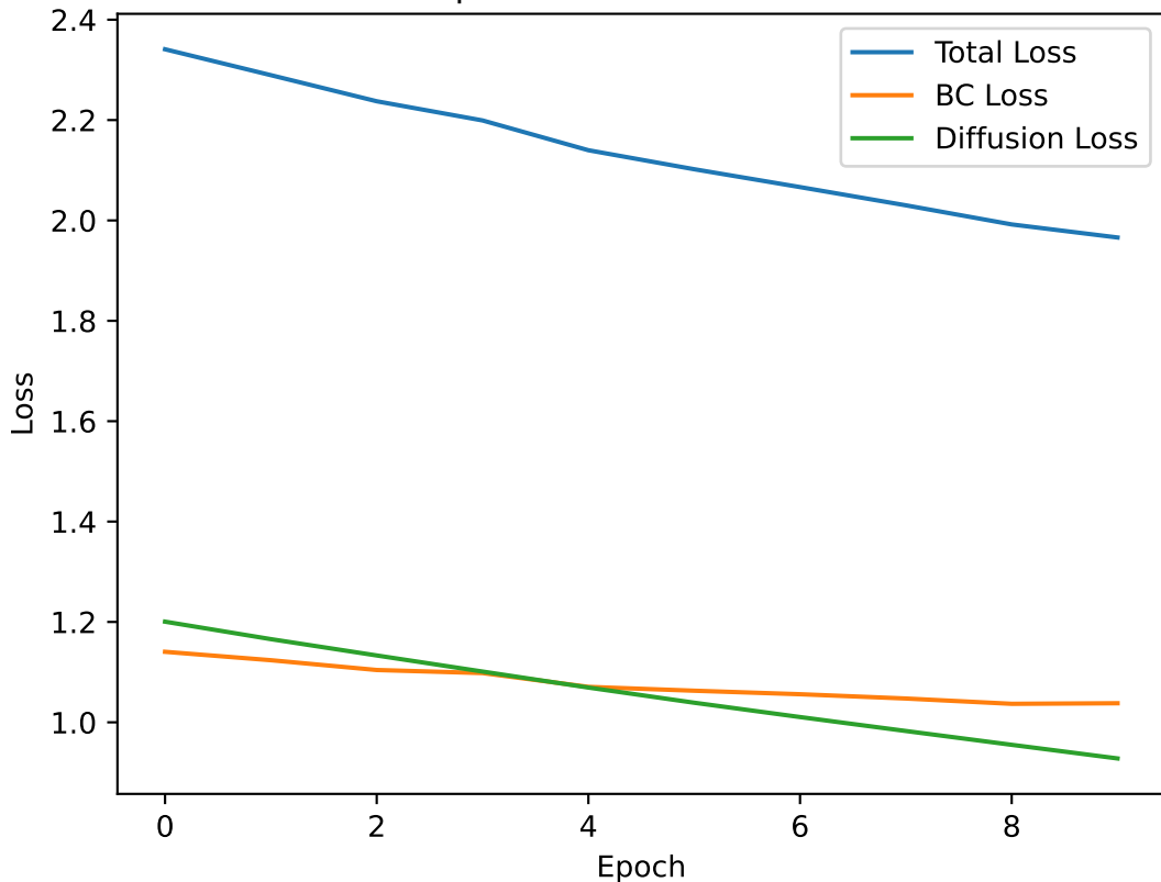
Experiment1: Loss Curves
