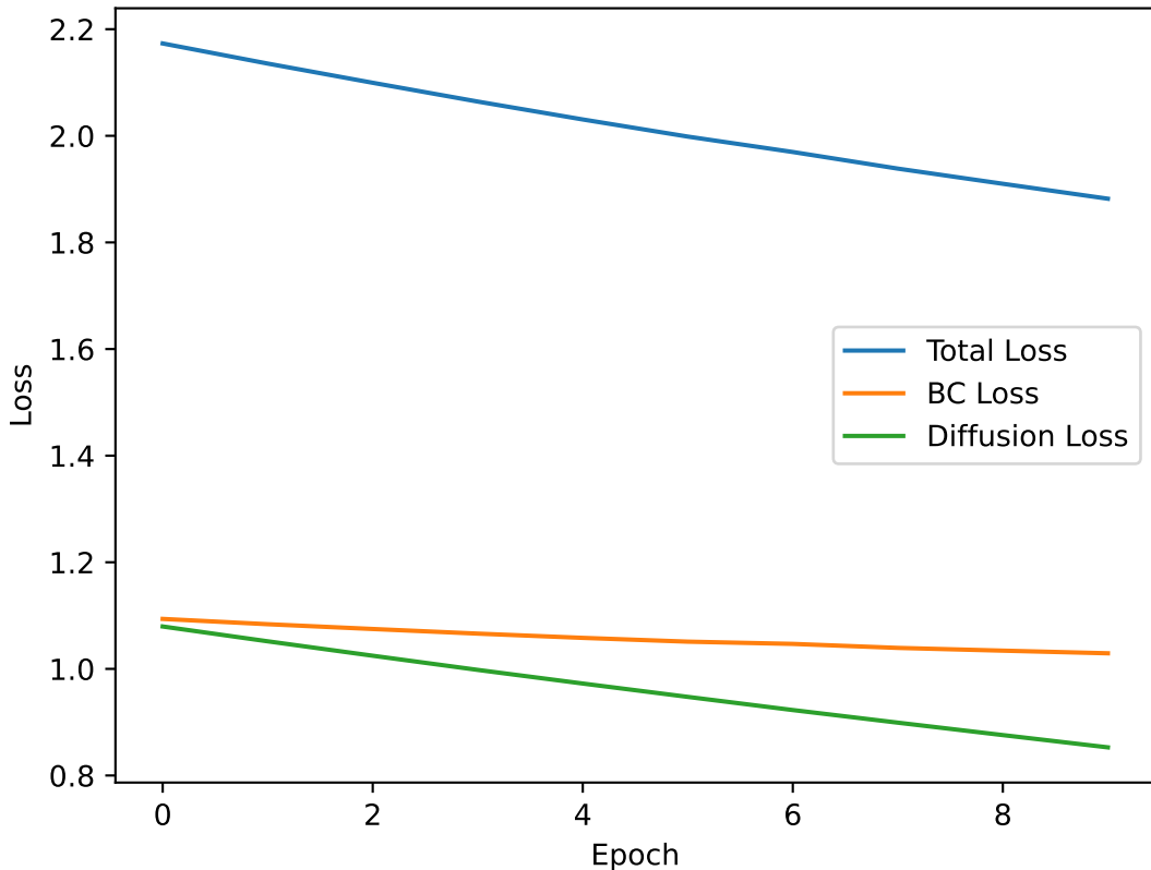
Experiment3: Loss Curves (Adaptive Noise)
