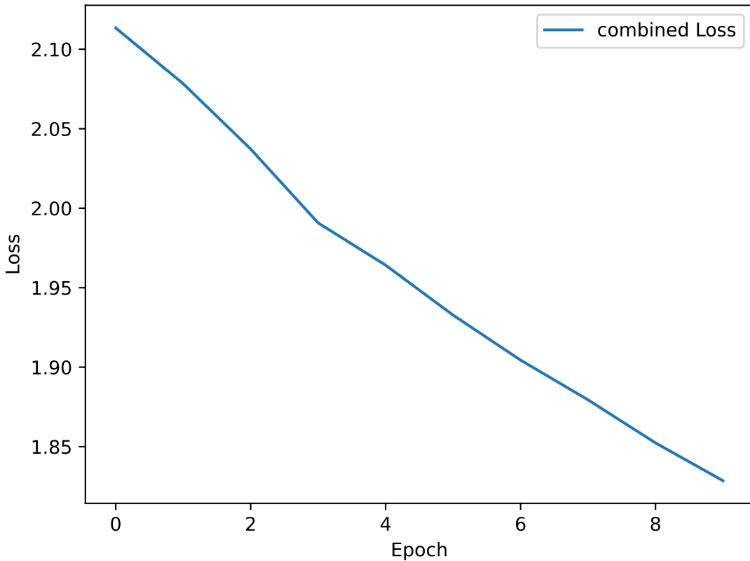
Experiment2: Loss Curve (combined)
