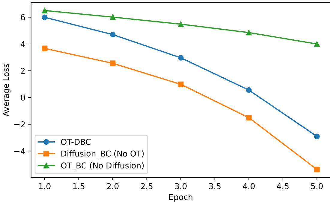
Training Loss (Loss Ablation Study)
