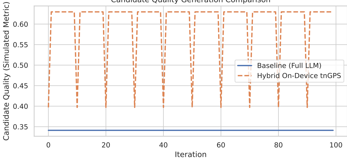
Candidate Quality Generation Comparison
