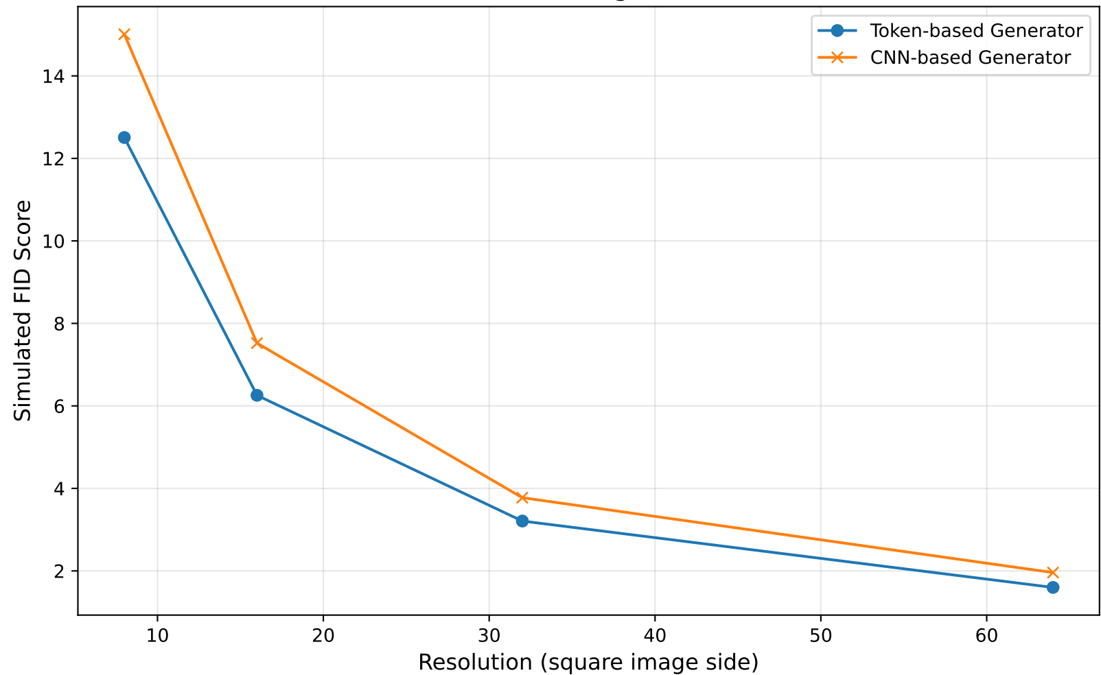
FID Score vs. Image Resolution
