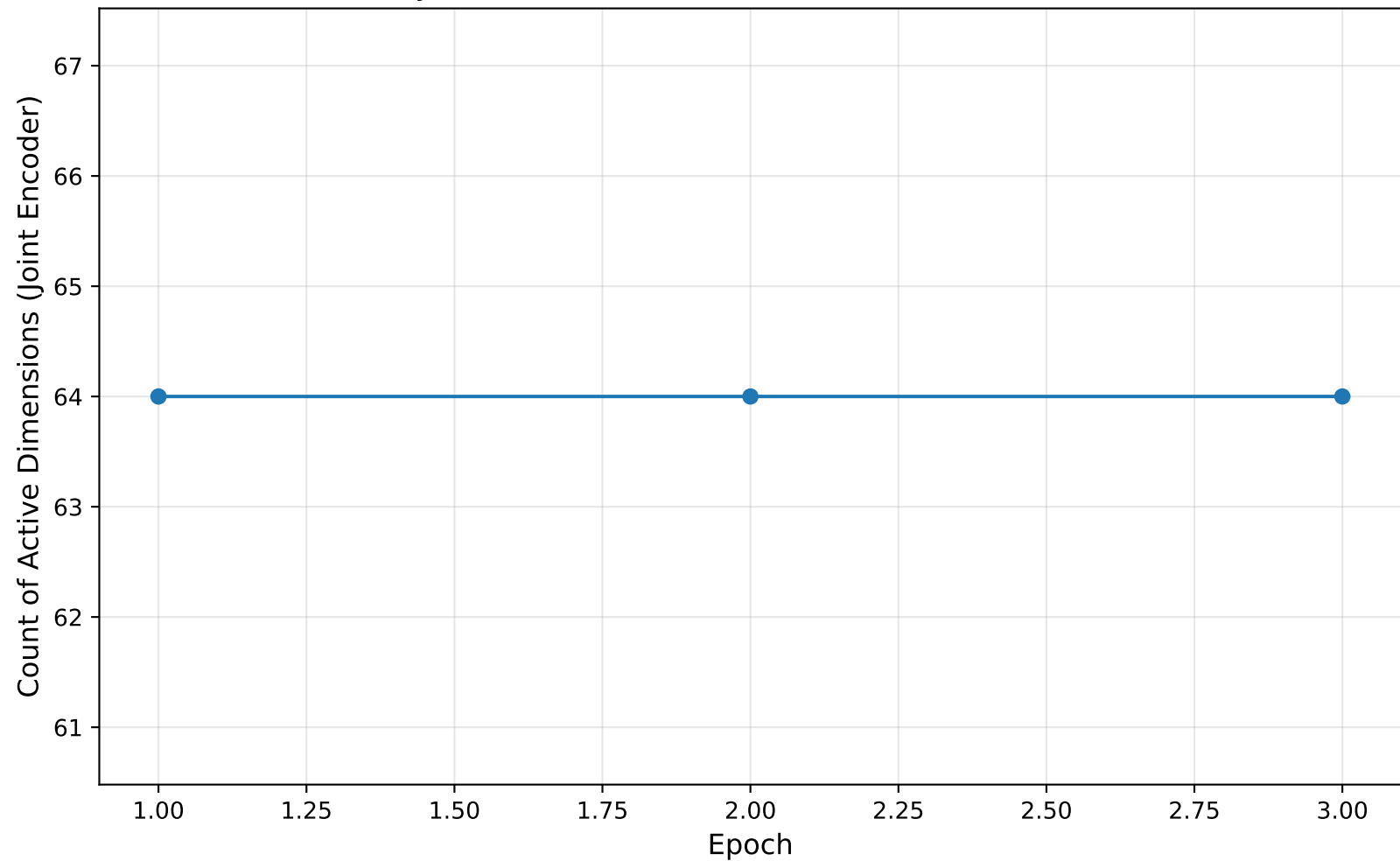
Joint Latent Active Dimensions Evolution
