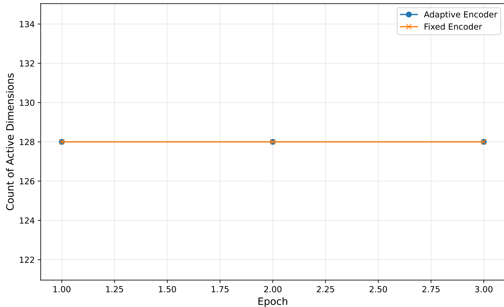
Latent Active Dimensions Evolution
