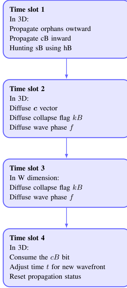
FIGURE 3 The Diffusion phase is composed of several time slots. It spreads all information necessary for relocation.
