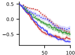
Hartmann (6D)
