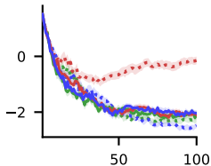
Branin (2D)
