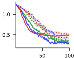
Ackley (5D)
