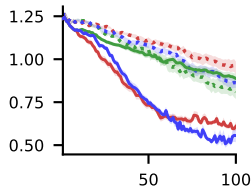
Ackley (8D)
