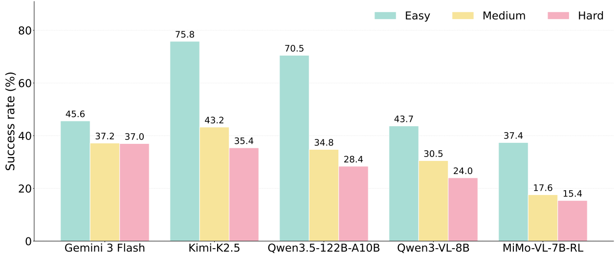
Figure 4 Success rate comparison across Easy, Medium, and Hard tasks. For readability, the figure visualizes representative models.
