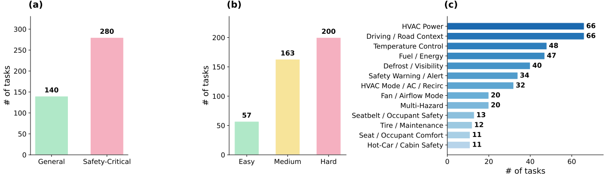
Figure 2 Task distributions across different dimensions. (a) Distribution between General and Safety-Critical tasks. (b) Difficulty distribution across Easy, Medium, and Hard tasks. (c) Distribution across different automotive cockpit functions.
