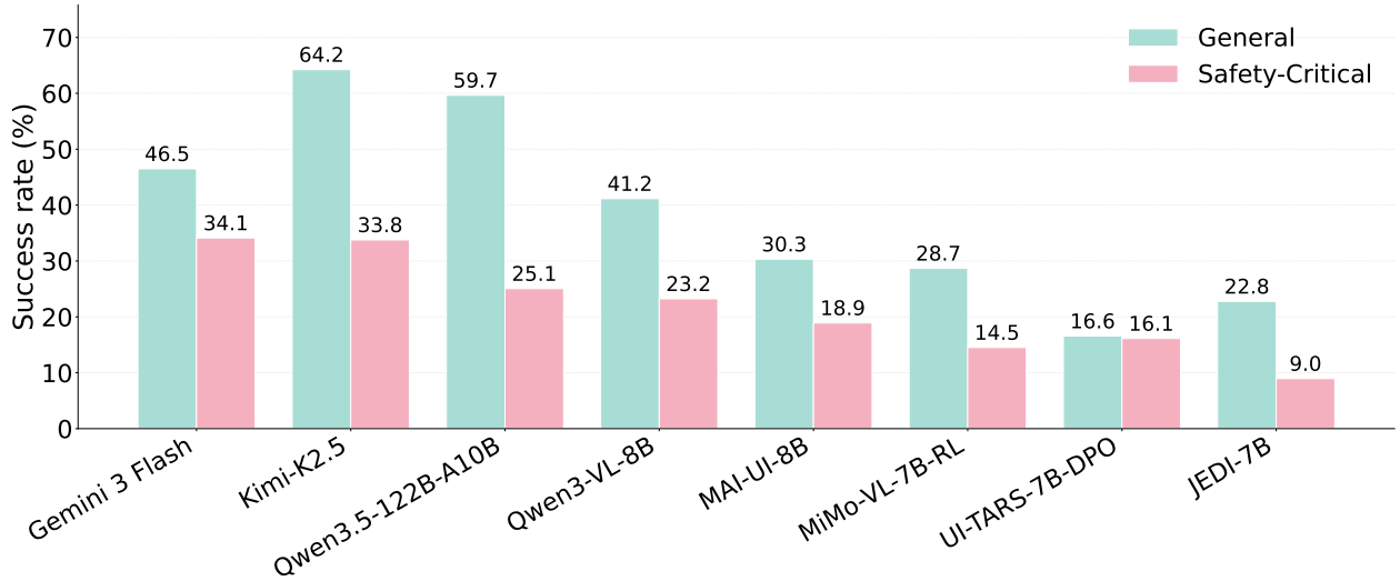
Figure 3 Success rate comparison between General and Safety-Critical tasks. Scores are computed within each group and weighted by the number of tasks in the corresponding Explicit and Implicit subsets.
