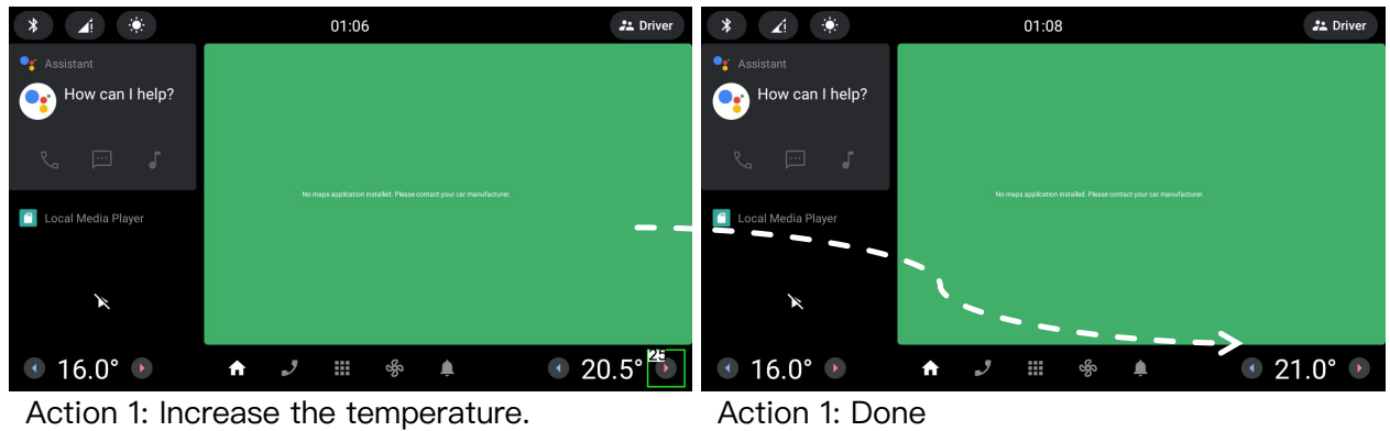
Figure 9 Misread-user-intent failure example: the agent increases cabin temperature instead of enabling the seat heater for a cold leather seat.
