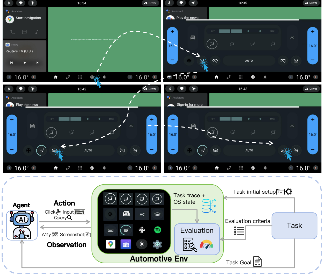
Figure 1 Overview of AUTOMOTIVE-ENV, an interactive benchmark for multimodal GUI agents in automotive cockpit systems. The environment couples screen-level cockpit interaction with vehicle-state signals: each task specifies an instruction and setup, the agent acts through UI actions and optional vehicle-state queries, and validators score the final system state and task trace.
