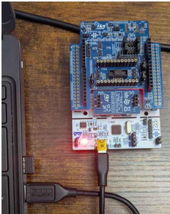
Figure 1: Physical setup of the STM32F401RE and X-NUCLEO-IKS4A1 board
